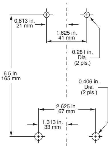
Mounting Dimensions
