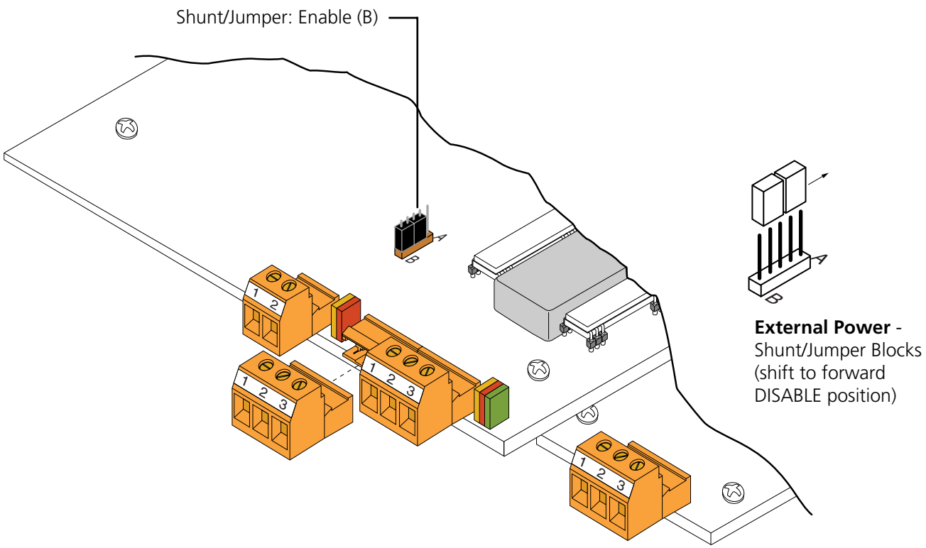
Detail - External Power Supply
