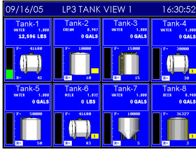
LP3 Tank View Display Up to 8 graphic tank representations may be displayed concurrently on each screen. (Scroll multiple display pages to view additional tanks.) A simple bar graph icon conveys tank level status at a glance, while total volumetric or mass is digitally displayed.
