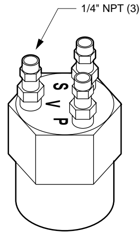
Tubing Connections
