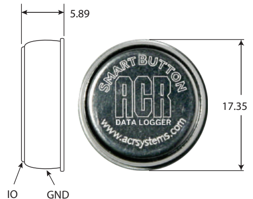
All dimensions shown are in millimeters
